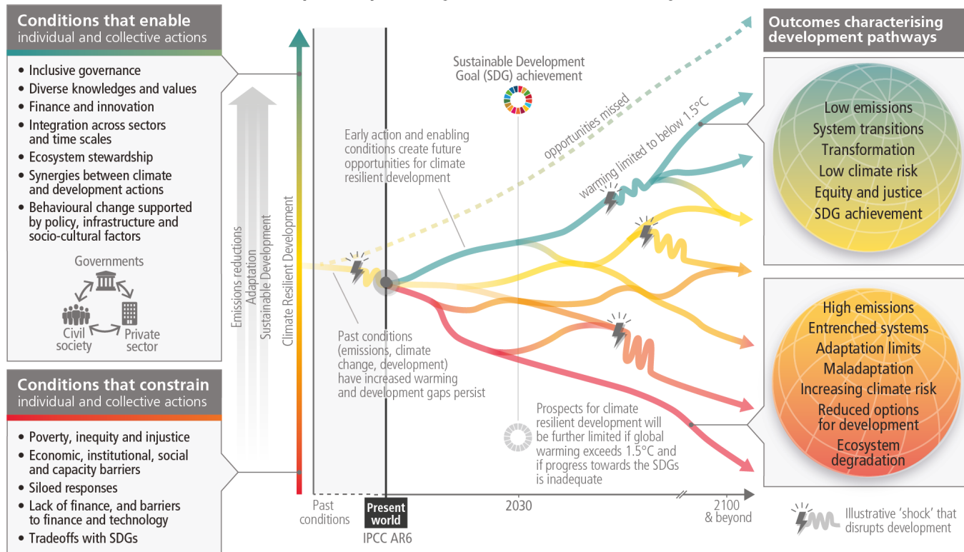
Source: Figure SPM.6, IPCC AR6 SYR
