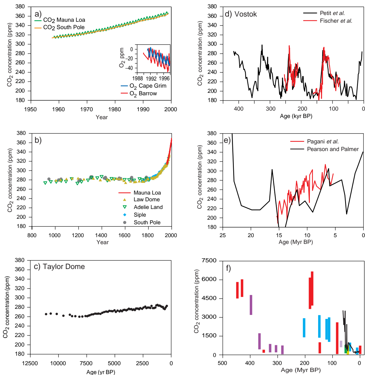
Figure 3.2: Variations in atmospheric CO 2 concentration on different time-scales. (a) Direct measurements of atmospheric CO 2 concentration (Keeling and Whorf, 2000), and O 2 from 1990 onwards (Battle et al. , 2000). O 2 concentration is expressed as the change from an arbitrary standard. (b) CO 2 concentration in Antarctic ice cores for the past millenium (Siegenthaler et al. , 1988; Neftel et al. , 1994; Barnola et al. , 1995; Etheridge et al. , 1996). Recent atmospheric measurements at Mauna Loa (Keeling and Whorf, 2000) are shown for comparison. (c) CO 2 concentration in the Taylor Dome Antarctic ice core (Indermühle et al. , 1999). (d) CO 2 concentration in the Vostok Antarctic ice core (Petit et al. , 1999; Fischer et al. , 1999). (e) Geochemically inferred CO 2 concentrations, from Pagani et al. (1999a) and Pearson and Palmer (2000). (f) Geochemically inferred CO 2 concentrations: coloured bars represent different published studies cited by Berner (1997). The data from Pearson and Palmer (2000) are shown by a black line. (BP = before present.)
