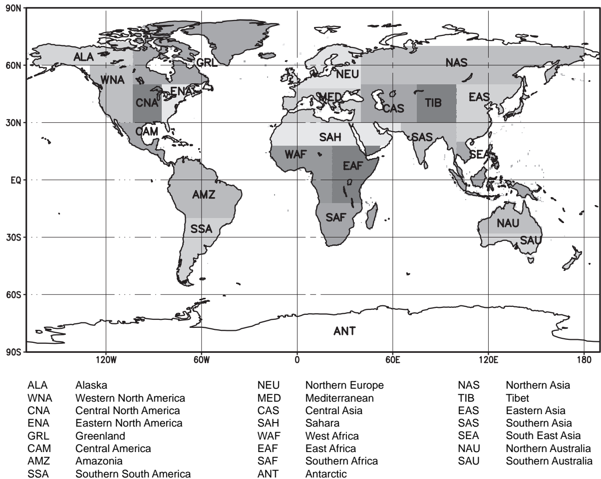
Figure 10.1: Regions used for the analysis presented in Figures 10.2 to 10.5 (from Giorgi and Francisco, 2000b).
