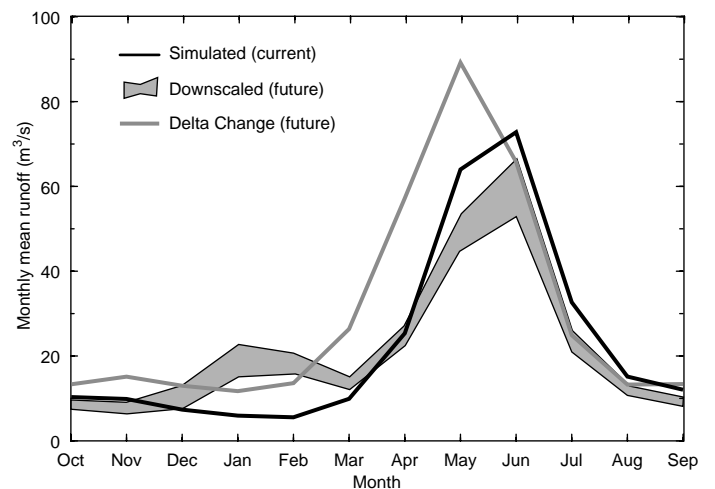
Figure 13.6: Differences in simulated runoff ( \text{m}^3/\text{s} ) based on a statistically downscaled climate scenario and a coarse resolution GCM scenario (labelled Delta Change) for the Animas River Basin in Colorado (modified from Hay et al. , 1999). The downscaled range (grey area) is based on twenty ensembles.
